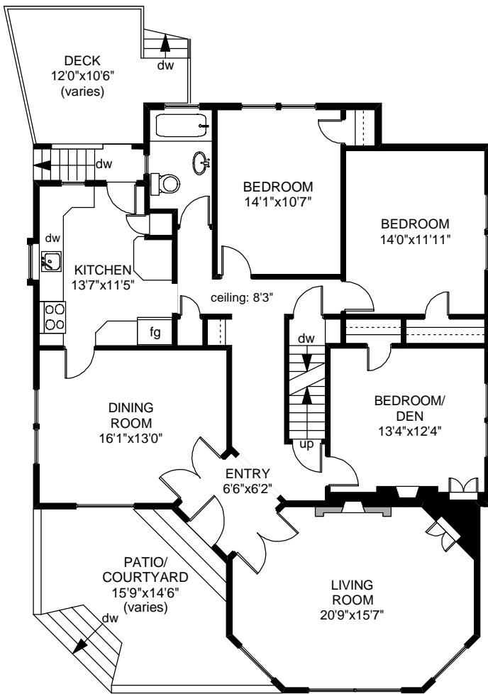
MAIN FLOOR 1599 SQ.FT
