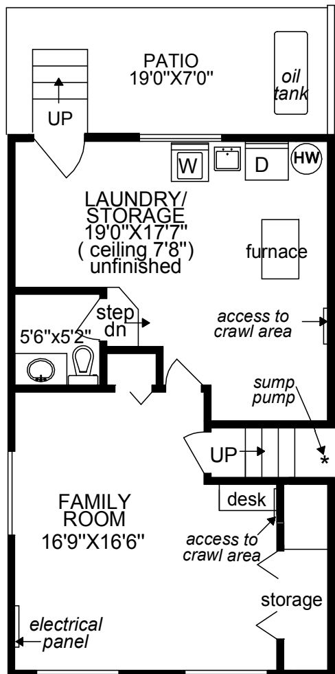
FLOOR 1 650 SQ. FT. (ceiling 7'8")
