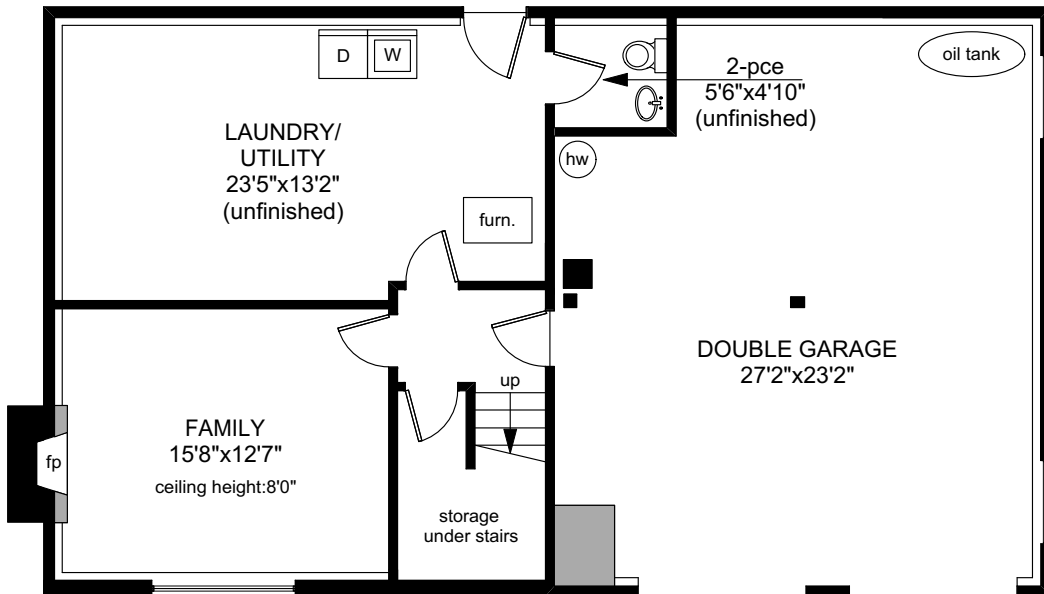
LOWER FLOOR 724 SQ.FT
